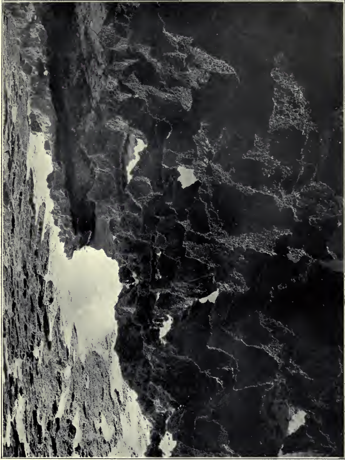
Erosion into knife-edged hollows of a bed of calcareous sandstone at high-tide level north of Dwarka headland.
