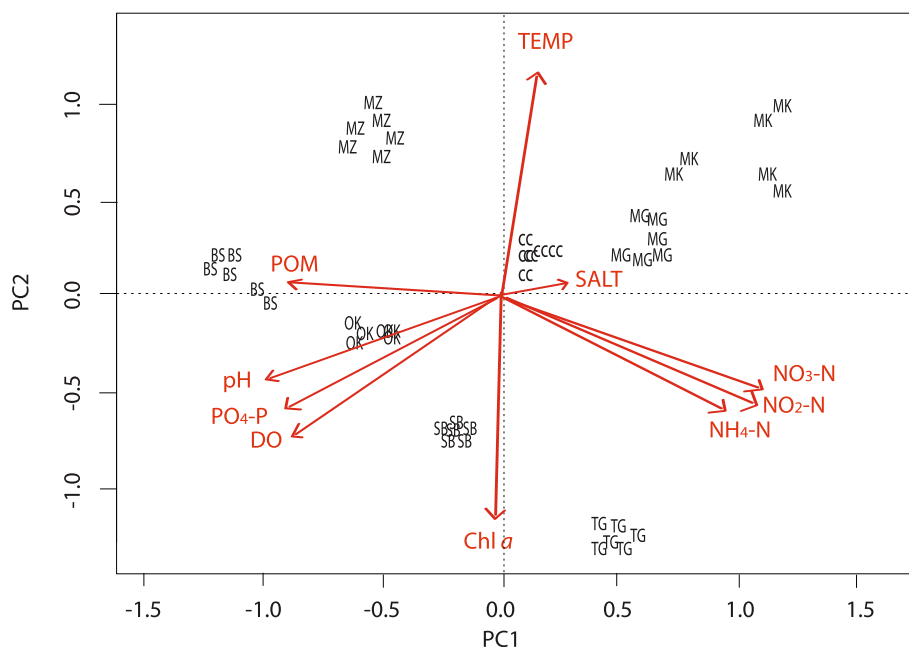
Figure 3 Principal component analysis of environmental data. MK, Makimato; CC, Convention Center; SB, Sunabe; MG, Mizugama; TG, Toguchi; MZ, Manza; BS, Bise; OK, Oku. PC1 = 43.17%; PC2 = 29.84%.
