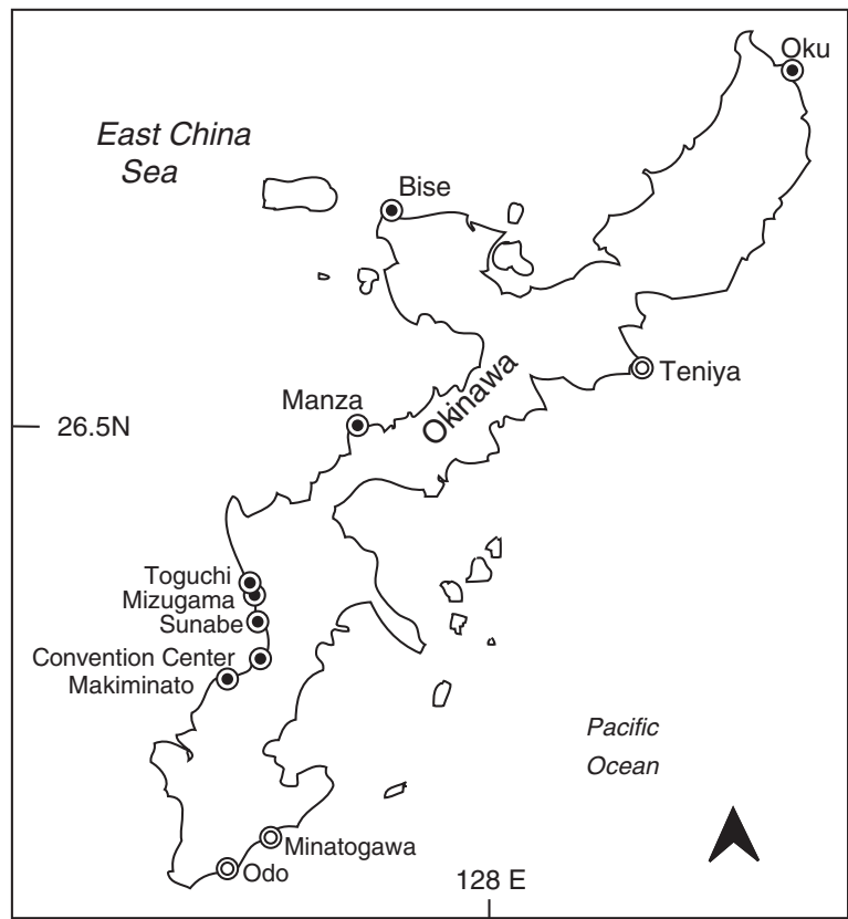
Figure 2 Map of sampling locations around Okinawa Island, Japan. Solid circles signify locations used in all analyses, white circles are additional locations where P. tuberculosa are abundant around Okinawa Island.
