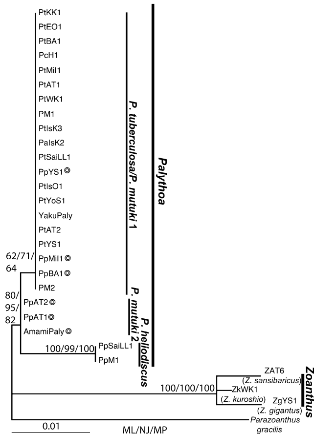
Fig. 3. Maximum likelihood tree of cytochrome oxidase I gene (COI) sequences. Values at branches represent ML, NJ, and MP bootstrap probability, respectively (>50%). Refer to Table 1 for sample name abbreviations.
